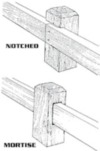
WOOD GUIDE RAIL
