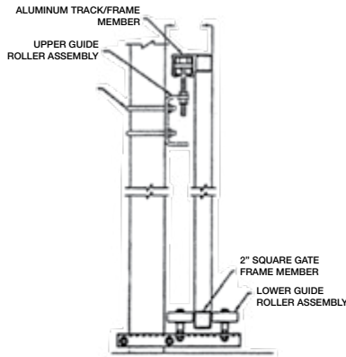
End View Upper & Lower Guide Roller Assembly Attached to Post
