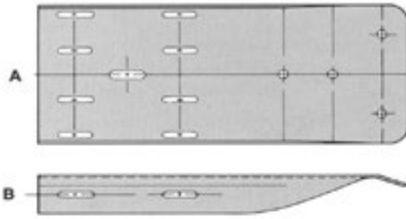
A — End Shoe, flat B — End Shoe, bent lip (for BCT)
