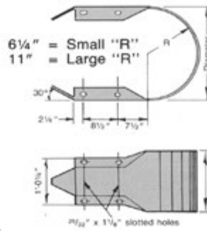
Double Buffer
