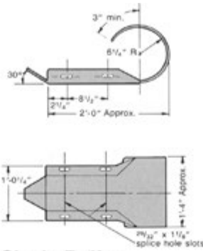
Single Buffer
