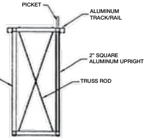
Box Frame 41'-0" to 50'-0"
